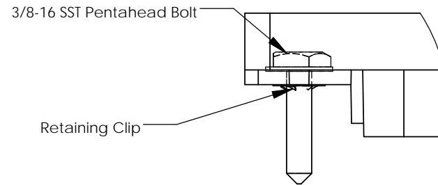
DETAIL A SCALE 1 : 2
